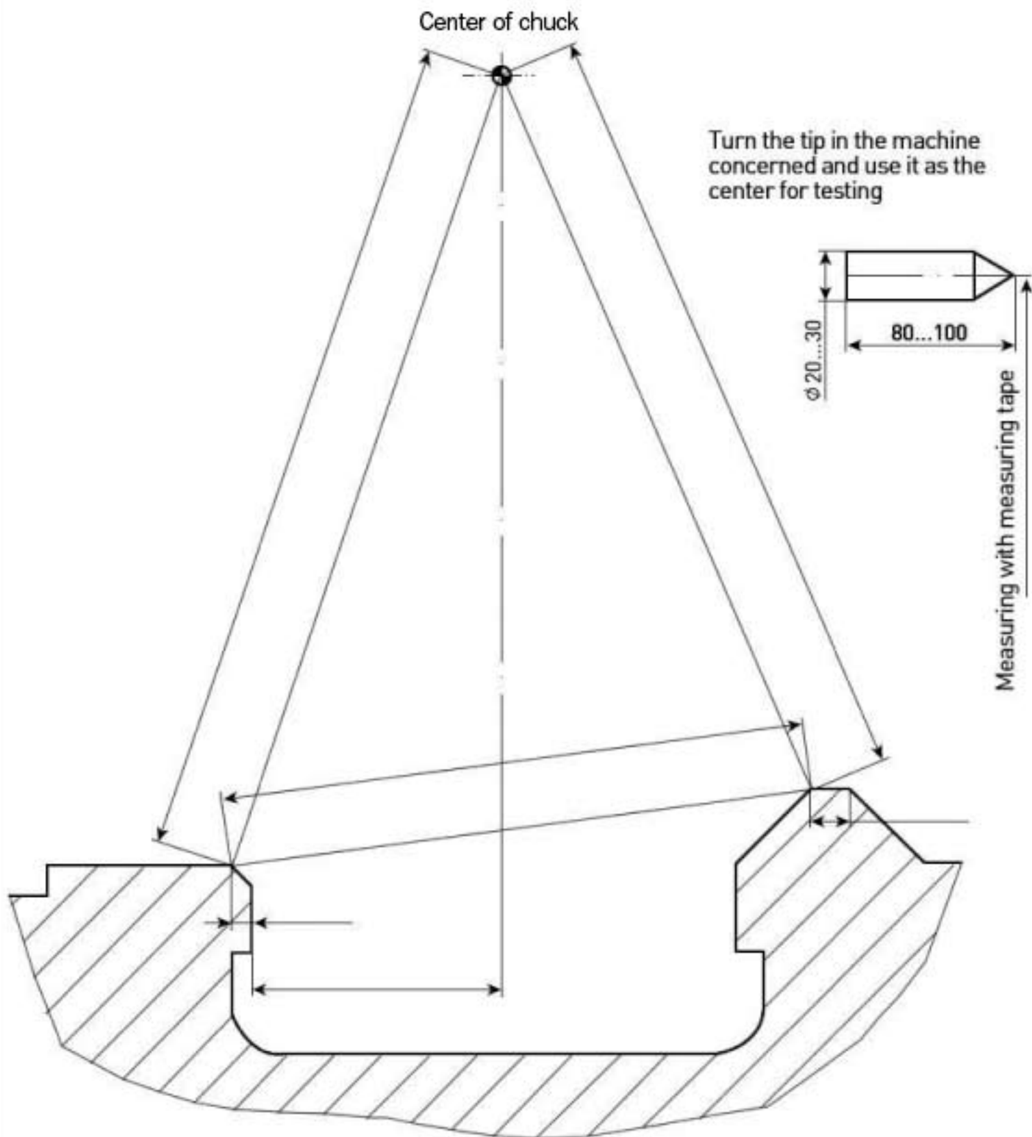
Dimension sheet for determination of pitch
